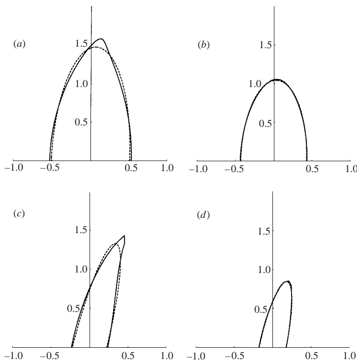
FIGURE 4. Vorticity contours (solid) and fitted ellipses (dotted) for experiment 2. Upper row: t = 57 , and (a) \omega = 0.25 \omega_0 (contour 6), (b) \omega = 0.55 \omega_0 (contour 12). Lower row: t = 63 , and (c) \omega = 0.7 \omega_0 (contour 15), (d) \omega = 0.85 \omega_0 (contour 18).
