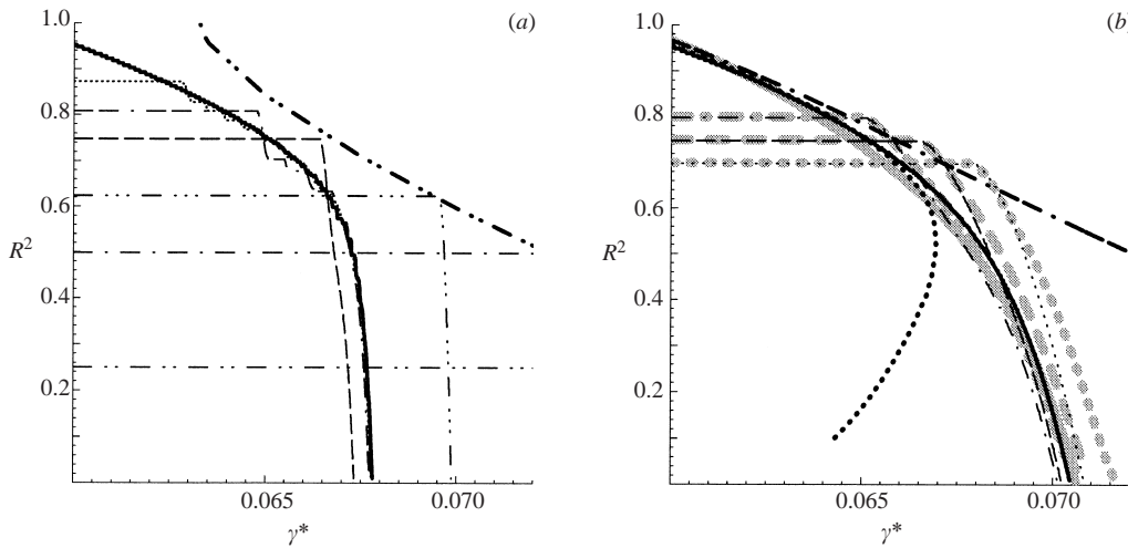
FIGURE 14. Erosion curves for truncated vortices. (a) EM+C for \tau = 20000 . —, R_i^2 = 1 ; \cdots , R_i^2 = 0.875 ; — · —, R_i^2 = 0.81 ; — —, R_i^2 = 0.75 ; — · · ·, R_i^2 = 0.625 ; — · · ·, turning line for the ‘mode-2’ perturbation in the EM. (b) CS and EM+C for \tau = 5000 . Thick grey lines, CS; thin lines, EM+C: —, R_i^2 = 1 ; — · —, R_i^2 = 0.8 ; — —, R_i^2 = 0.75 ; \cdots , R_i^2 = 0.7 ; \cdots , stationary corner branch in the EM+C; — · · ·, turning line for the ‘mode-2’ bifurcation in CS.
