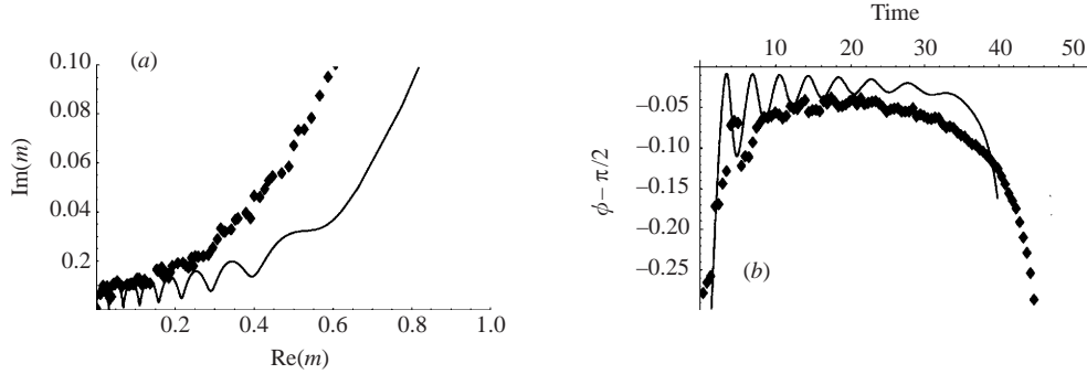
FIGURE 7. (a) Solid line: evolution of the solution to (3.1) in the m -plane for \omega = 0.6 \times 2\pi and 1/\tau = 0.000014 ; \blacklozenge , m(t) calculated for the contour \omega = 0.6 \times 2\pi in experiment 1. (b) Same as (a) except the evolution of \phi - \pi/2 is shown.
