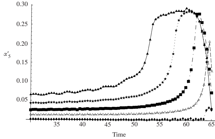
FIGURE 5. Residual fifth-order moment |\alpha'_5| as a function of time ( t > 30 ) for various vorticity contours in experiment 2: \blacklozenge , \omega = 0 (contour 1); \blacktriangle , \omega = 0.2\omega_0 (contour 5); \blacksquare , \omega = 0.45\omega_0 (contour 10); \star , \omega = 0.7\omega_0 (contour 15); and \blacktriangle , \omega = 0.95\omega_0 (contour 20).
