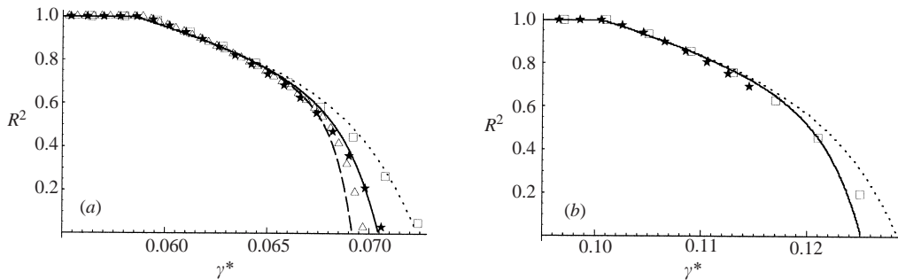
FIGURE 10. (a) Erosion of the vortex as shown by the mean-squared radius of the separatrix after the onset of erosion as a function of the normalized strain \gamma^* (note: R^2 = 1 before the onset of erosion). For CS: \square , \tau = 1250 ; \star , \tau = 2500 ; \triangle , \tau = 5000 . For EM+C: ···, \tau = 1250 ; —, \tau = 2500 ; —·—, \tau = 5000 . (b) The same for the pure strain case. For CS: \square , \tau = 500 ; \star , \tau = 1000 . For EM+C: ···, \tau = 500 ; —, \tau = 1000 .
