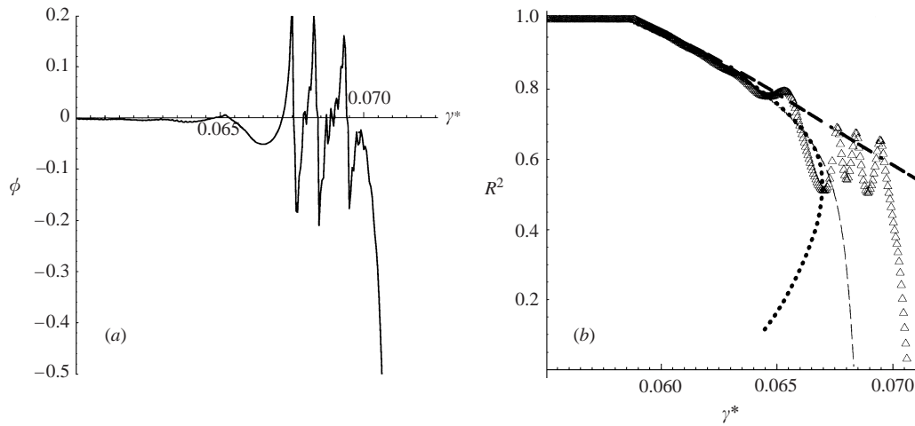
FIGURE 15. Oscillations of the vortex as it passes the ‘mode-4’ bifurcation during the erosion in a CS simulation with \tau = 10000 . (a) Oscillations of the orientation \phi of the vortex core as a function of \gamma^* . Compare with figure 9. (b) \Delta , Radius of the vortex (defined as in figure 10). Other curves are as in figure 12(a).
