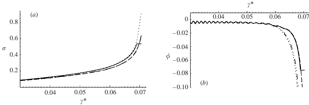
FIGURE 9. (a) Evolution of the eccentricity as a function of the strain for \tau = 2500 . For CS: —, \sigma(0) ; ···, \sigma(0.6) . For EM+C: —·—, \sigma(0) ; —, \sigma(0.6) . (b) Evolution of the orientation \phi for the same case. The EM+C curves for the radius r = 0.6 level off after the elimination of this contour.
