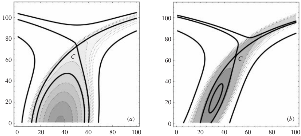
FIGURE 6. (a) Enlargement of the vorticity chart at t = 42 for experiment 1. Thick solid line: the separatrices, crossing at the critical point C , and other selected streamlines. Dotted line: vorticity contours with contour interval 0.1\omega_0 . Axis labels are in units of the collocation grid. (b) Same but at t = 48 and with a contour interval 0.2\omega_0 . The enlarged window has the same size in (a) and (b) but has a different centre.
