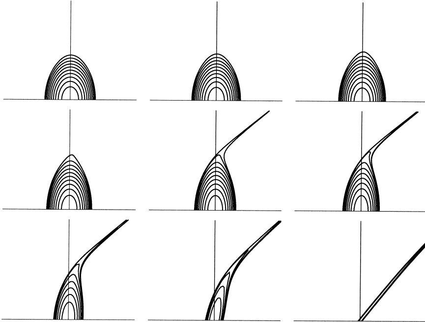
FIGURE 3. Vorticity charts at times t = 42, 45, 48, 51, 54, 57, 60, 63, 66 from left to right and top to bottom for experiment 2, conducted using the CS method. The vortex is initially parabolic and is subjected to a linearly growing pure shear. All 20 contours are plotted but several contours at the vortex edge have become indistinguishable as a result of stripping.
