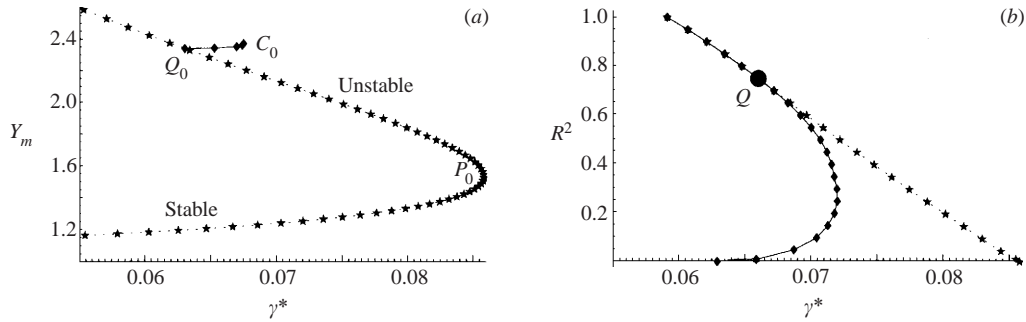
FIGURE 13. (a) Detail of the bifurcation diagram of the stationary vorticity patch within an adverse shear where Y_m is the semi-major axis length of the vortex. Dotted line and \star : elliptical solution exhibiting a regular turning point at P_0 . Solid line and \blacklozenge : branch bifurcating from the mode-4 instability on the unstable elliptical branch at Q_0 and leading to a corner patch solution at C_0 which is also a regular turning point. Another branch, not shown, extends the solid line across Q_0 , leading to a peanut shaped solution. (b) Stability diagram of the CS equilibrium states within an adverse shear obtained by continuation as indicated in the text. Dotted line and \star : \gamma^* = \gamma_m(R) , the regular turning point of the mode-2 instability. Solid line and \blacklozenge : \gamma^* = \gamma_4(R) , the mode-4 instability. The two curves are tangent at Q ( R^2 = 0.75, \gamma^* = 0.6589 ).
