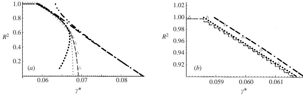
FIGURE 12. Erosion curves and limit branches of stationary solutions. (a) \Delta , Erosion curve for CS and \tau = 5000 ; —, erosion curve for the EM+C and \tau = 5000 ; \cdots , erosion curve for the EM+C and \tau = 20000 ; - - -, turning line of the mode-2 bifurcation in CS; - · · -, turning line of the mode-2 bifurcation in the EM; \cdot \cdot \cdot , branch of stationary solutions with corners in the EM+C. (b) Enlargement of the upper left part of (a) near R = 1 .
