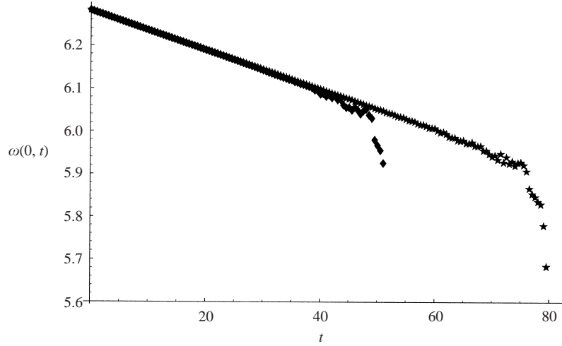
FIGURE 16. Evolution of the maximum vorticity at the centre of the vortex. \blacklozenge , experiment 1; \star , same as experiment 1 but with half the strain growth rate. Solid line, curve predicted by (6.3).
