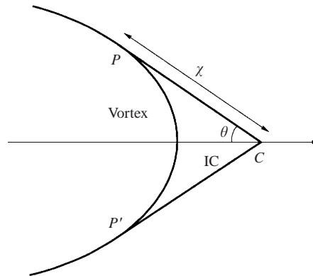
FIGURE 8. Sketch of the corner near the critical point as idealized for use in the EM+C.
