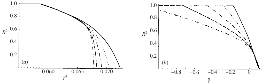
FIGURE 11. (a) Erosion curves for the EM+C defined as in figure 10. —, \tau = 1250 ; \cdots , \tau = 2500 ; - - -, \tau = 5000 ; - · - ·, \tau = 10000 ; - - - - , \tau = 20000 . (b) The same after rescaling \gamma^* into \tilde{\gamma} = (\gamma^* - \gamma_c)(\tau\omega_0)^{2/3} .
