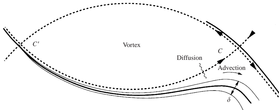
FIGURE 17. Separation of the boundary layer from an eroding vortex.
