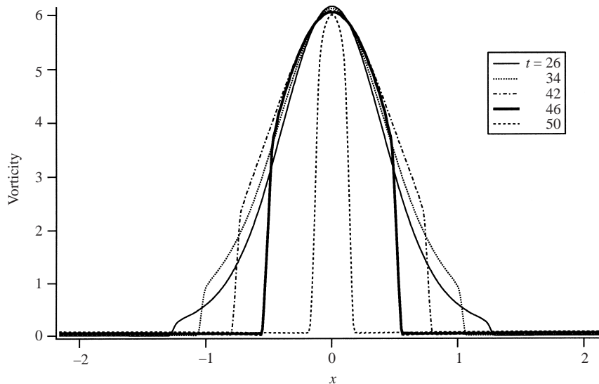
FIGURE 2. Vorticity section along the x -axis for experiment 1 at several times as indicated in the legend.
