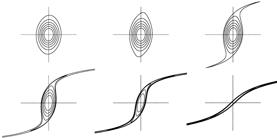
FIGURE 1. Vorticity charts at times t = 26, 31, 36, 41, 46, 51 from left to right and from top to bottom for experiment 1, conducted using the PS method with a small viscosity. The vortex is initially Gaussian and is subjected to a linearly growing adverse shear. The contour interval is 0.8.
